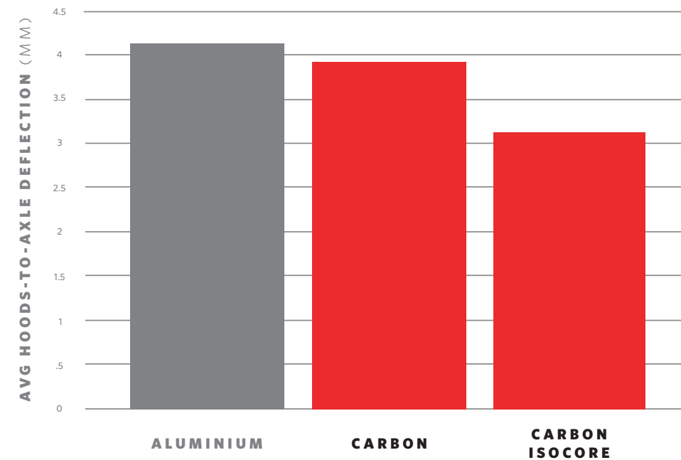
AVERAGE HOODS-TO-AXLE DEFLECTION
