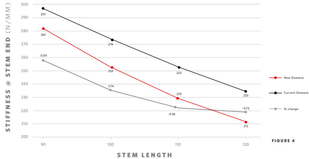
FRONT END STIFFNESS COMPARISON (@ STEM END)
